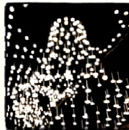
Blackbody
